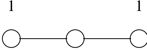
Figure 5: The SU(4) Dynkin diagram where the numbers indicate the Dynkin labels of the representation. The roots u_j are associated with one outer root, v_j with the other outer root, and r_j with the middle root.
