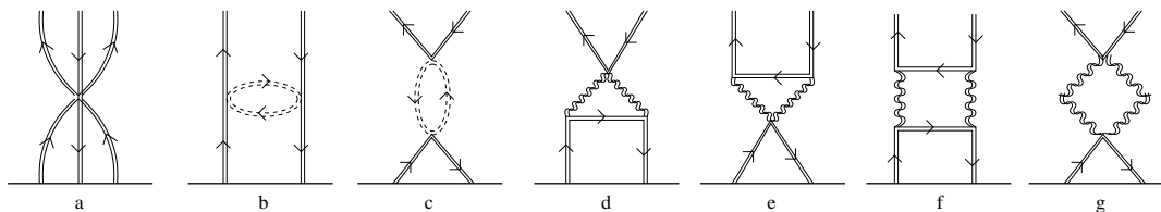
Figure 2: The planar diagrams that contribute to operator mixing at two loops. The horizontal bar denotes the operator. The directions of the arrows refer to the flow of the SU(4) flavor. Since the superpartners of the scalars are in the conjugate representation of SU(4), the fermion arrows in (b) and (c) have the opposite orientation. The gauge propagators in (d), (e), (f) and (g) do not have arrows since they do not carry SU(4) charges. It turns out that only (a), (b) and (d) contribute to the anomalous dimension.
