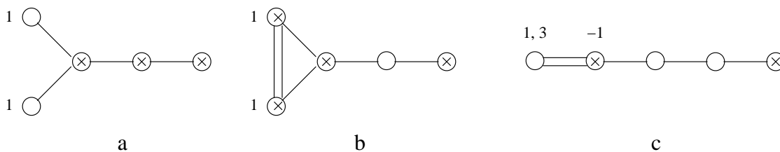
Figure 8: Other OSP(2, 2|6) Dynkin diagrams.
