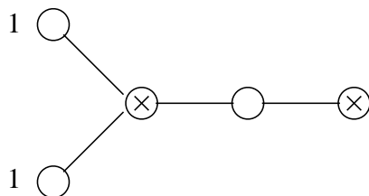
Figure 7: A different choice for the OSp(2, 2|6) Dynkin diagram with two fermionic roots.
