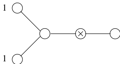
Figure 6: One choice for the OSp(2, 2|6) Dynkin diagram. The Dynkin labels are taken from the SU(4) spin chain.
