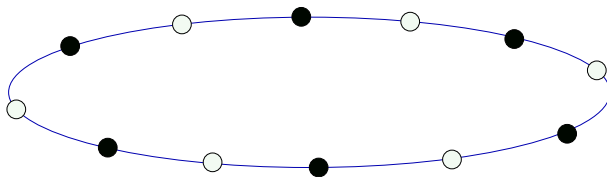
Figure 1: The alternating spin chain.
